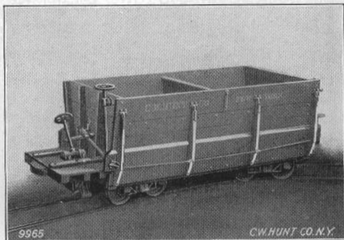
No. 9965. Cable Coal Car.
