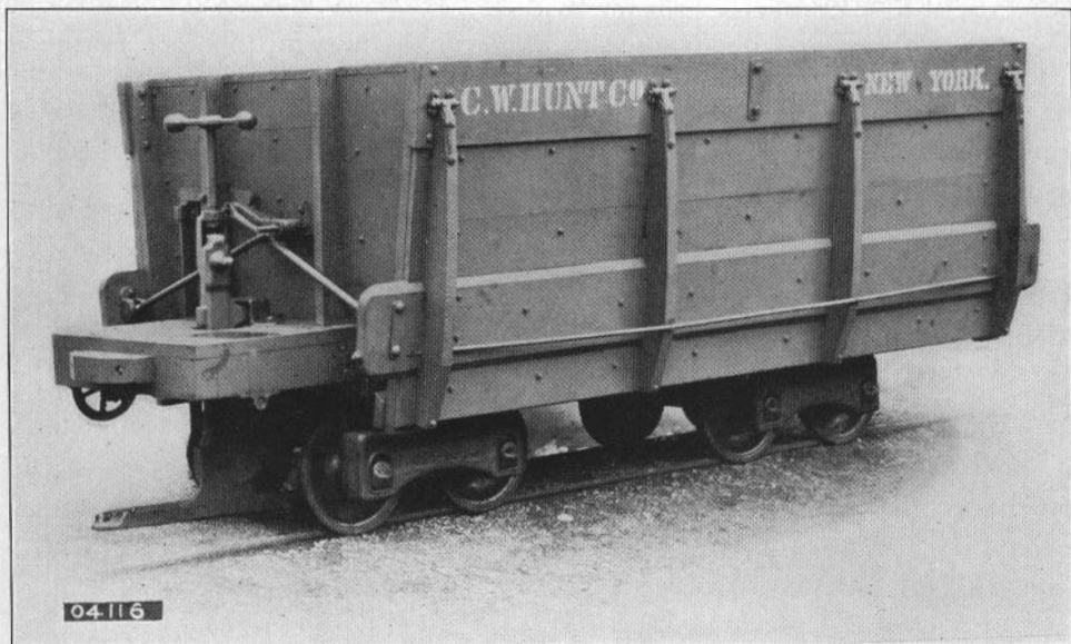
No. 04116. Two-ton Cable Car for Heavy Cable Railways. This car has the bottom inclined each way to the sides which open and dump the load on both sides of the track.
